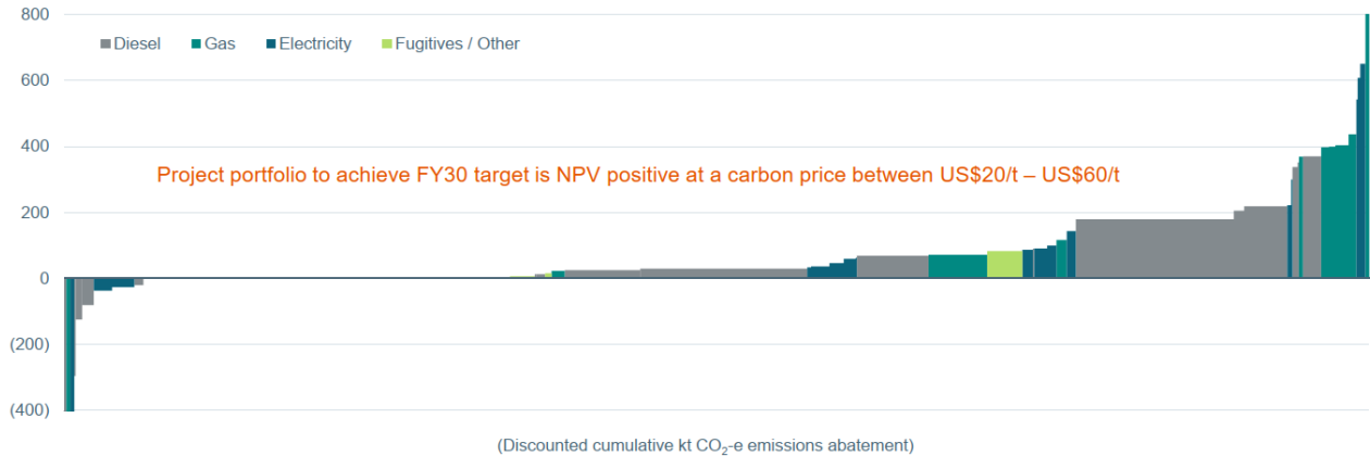
Marginal Abatement Cost Curve 1 (US$/tCO 2 -e)
